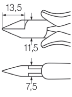
wide, pointed head with bevelled edge Z 41 1 04
